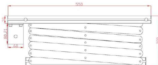
CLOSED LIFT: SIDE VIEW
