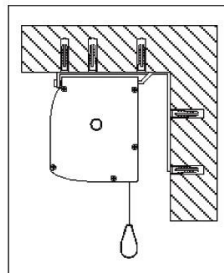
Ceiling Mounting
