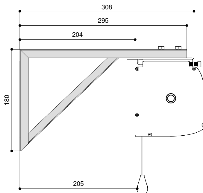
SUPPORT LONG : L = 295mm
